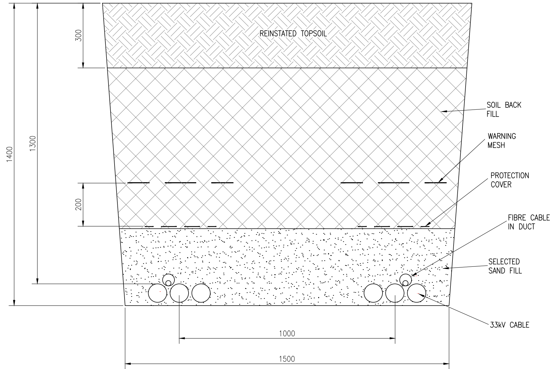
TYPICAL CABLE TRENCH (SCALE 1:10)
